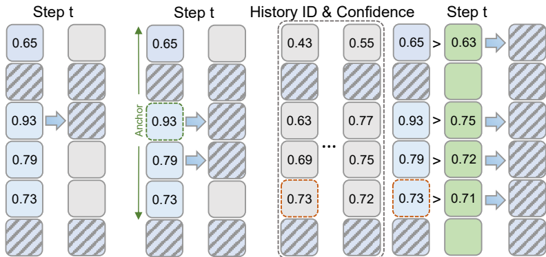
(a) Top-1 Decoding (b) Anchor Decoding (c) Spatio-Temporal Aware Decoding
